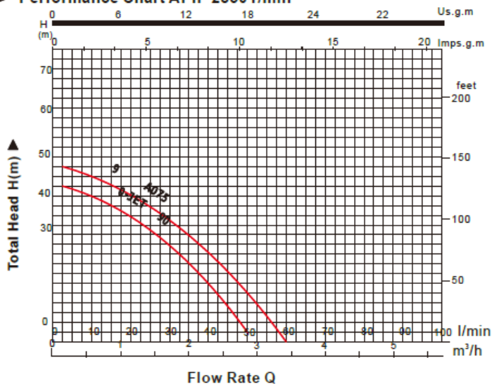
► Performance Chart AT n=2850 r/min
